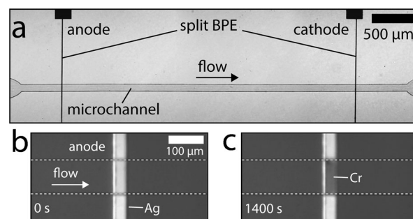
Figure 9. a) Optical micrograph of a microfluidic channel that incorporates a split BPE for streaming potential experiments. The channel was 6 mm long and the BPE consisted of two Au microbands making l_{\text{elec}} = 4.5 mm. b) An optical micrograph of the BPE anode, which was modified with a 20 nm thick layer of Ag over 5 nm of Cr. The channel contained an aqueous 1.0 mM benzoquinone solution. At t = 0 s, the two poles of the BPE were connected externally. c) After 1400 s, the Ag film was completely oxidized. Adapted with permission from Ref. [41]. Copyright 2011 American Chemical Society.
